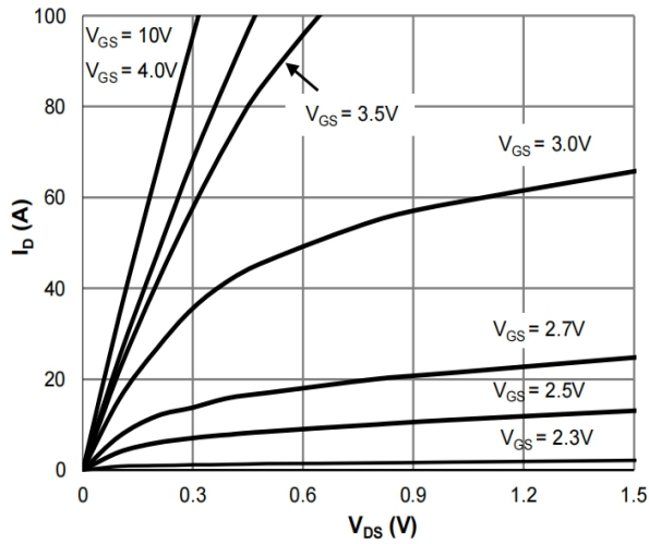
Figure 1: Saturation Characteristics
